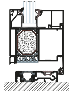
EI 30 bottom section with threshold
