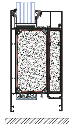
EI 60 bottom section with kick-plate
