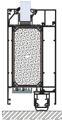
EI 30 bottom section with falling threshold
