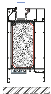
EI 30 bottom section with kick-plate
