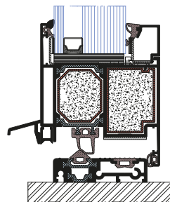
EI 30 bottom section with threshold
