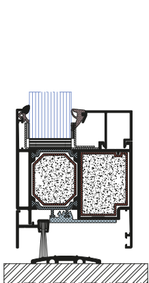
EI 60 bottom section with brush seal
