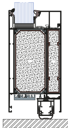
EI 60 bottom section with falling threshold
