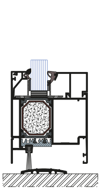
EI 30 bottom section with brush seal
